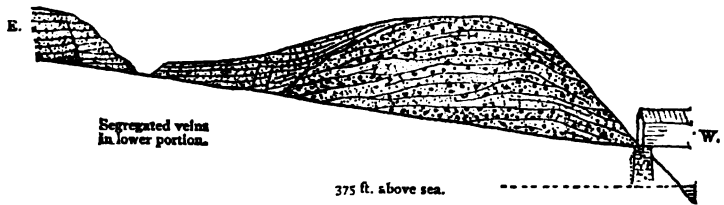
FIG. 88.—Section east from Ledyard Bridge, Hanover, New Hampshire, showing segregated veins in the lower portion. Length, about seven hundred feet. Height of kame above the river, one hundred and forty feet. (Upham.)
